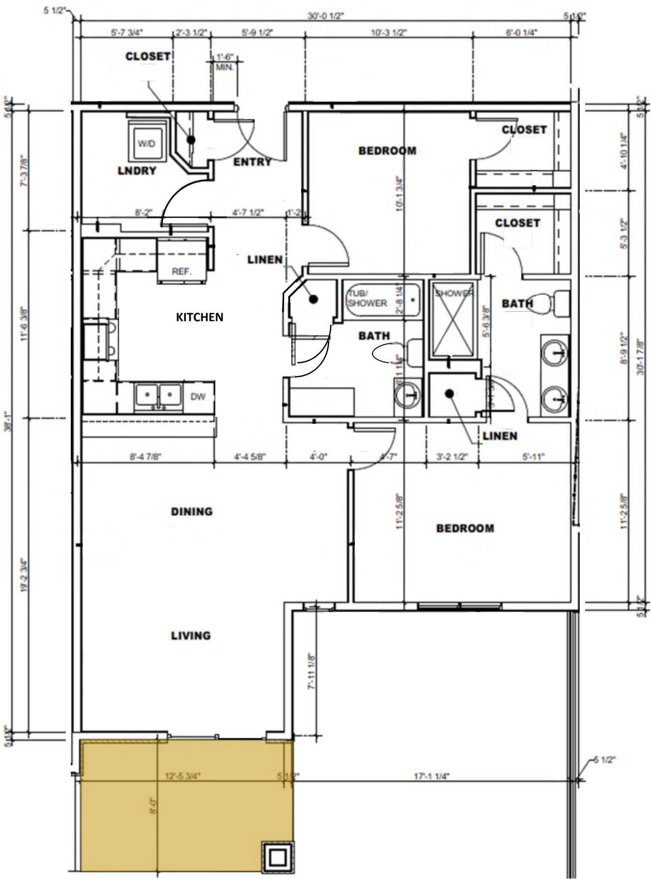
Layout 2C 992 SF (Units 116, 216, 316)
