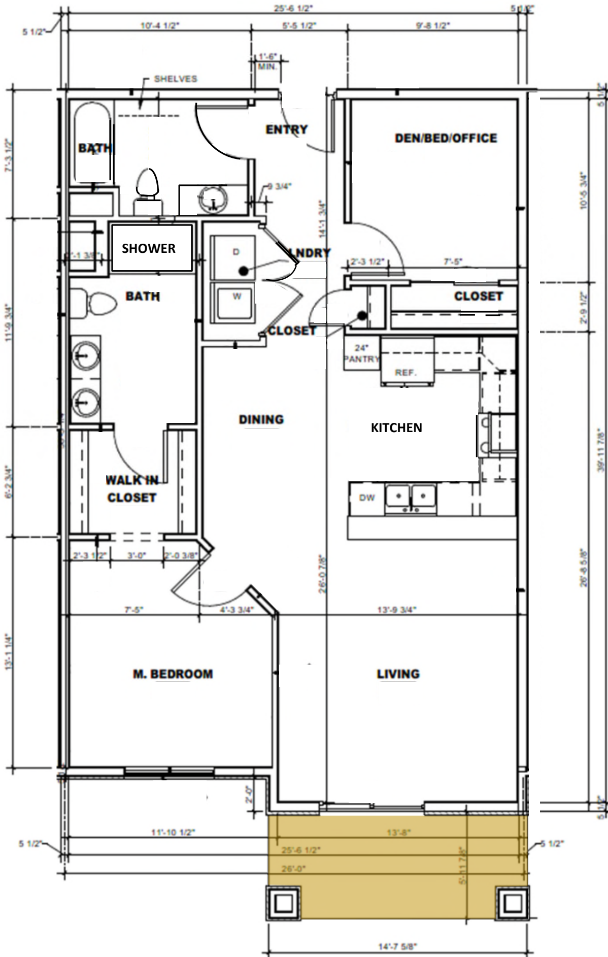
Layout 2B.1 988 SF (Units 111, 209, 211, 309, 311)
