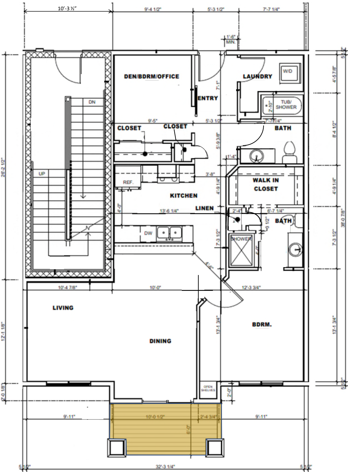
Layout 2D 974 SF (Units 204, 304)
